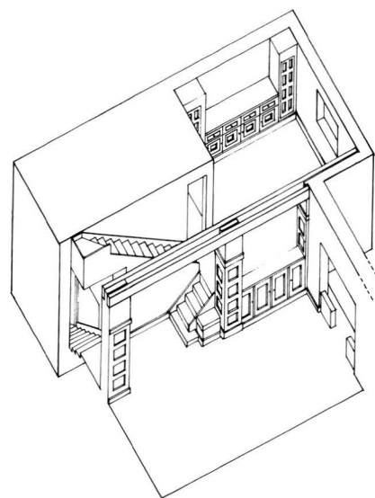
19. Rufer House, axonometric view of the stairway and dining room. Drawing by Laurel Ulland.
