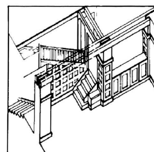
27. Rufer House, axonometric vignettes demonstrating the potential for simultaneity within the wall assembly. Drawings by Julie Oseid.
